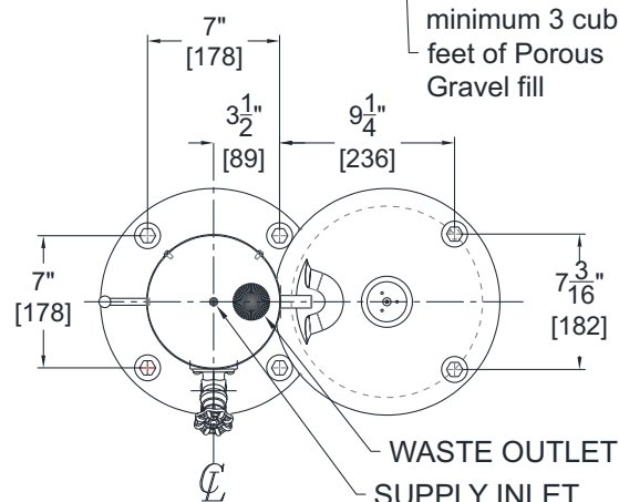
MOUNTING BASE DETAIL
